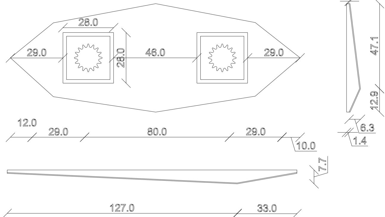
SPECCHIO VISTA RETRO / rear view mirror
